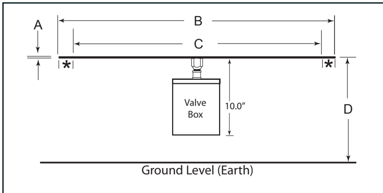
Figure 1. Flat Disc Dimensions; refer to Table 1. *( 2.00" minimum overlap per side required to secure disc)
