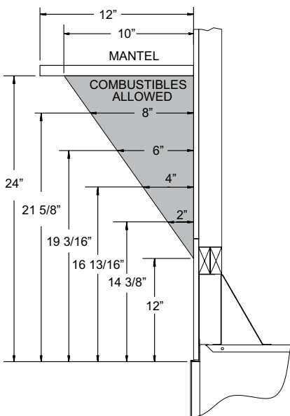
Figure 2 - Mantel Clearances
