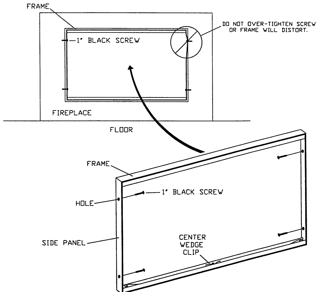
1 - FRAME INSTALLATION
