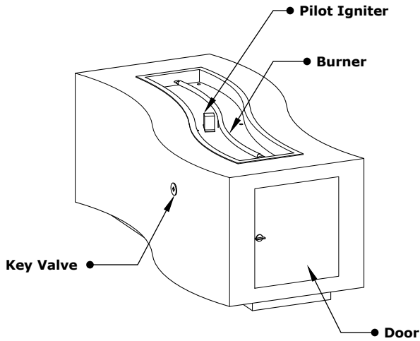
ISOMETRIC VIEW
