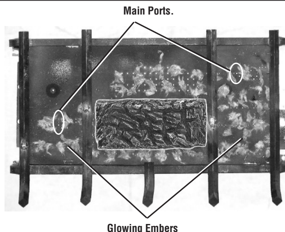
Figure 65—Glowing Ember Placement
