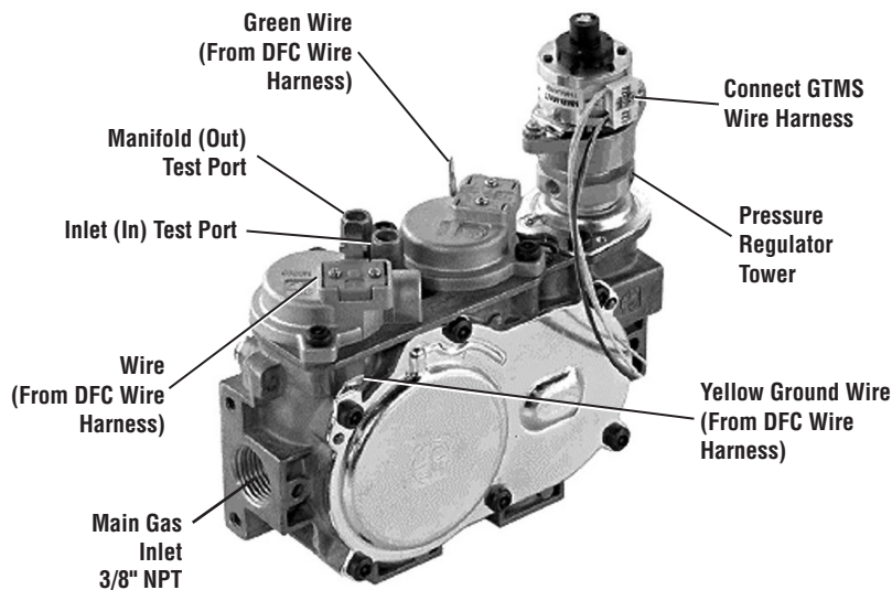
Figure 60—SIT Proflame Valve
