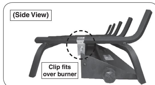
Fig. 10-3 Grate placement detail
