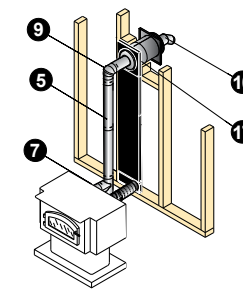
Through-the-Wall with Vertical Rise
