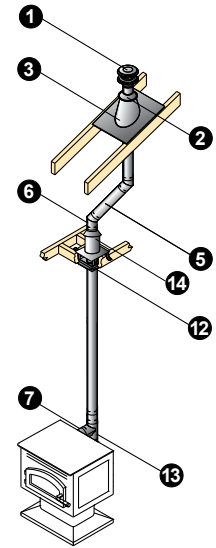
Attic Offset
