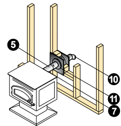
Through-the-Wall
