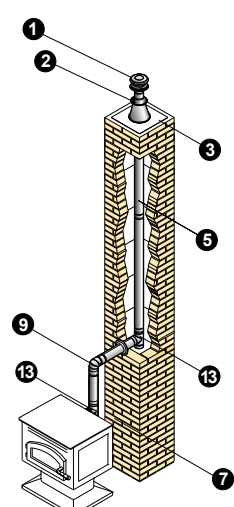
Masonry Chimney Relining
