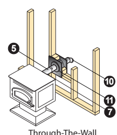
Through-The-Wall
