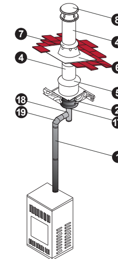
Oil Furnace
