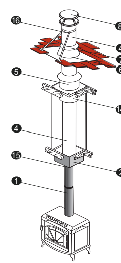
Multi-Story
