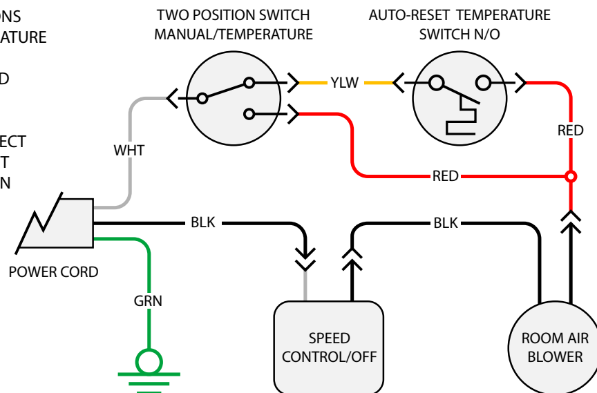
Figure 34 - Blower Wiring Schematic
