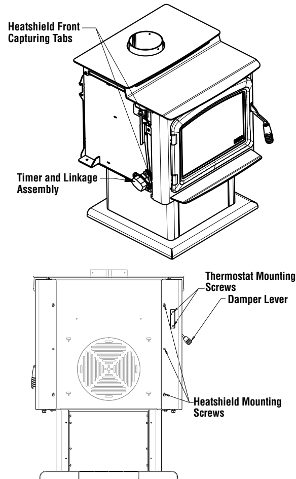
Figure 27b - Timer Replacement / Adjustment
