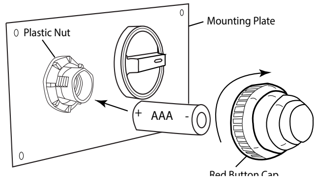
Fig. 9 Installing battery into Piezo.
