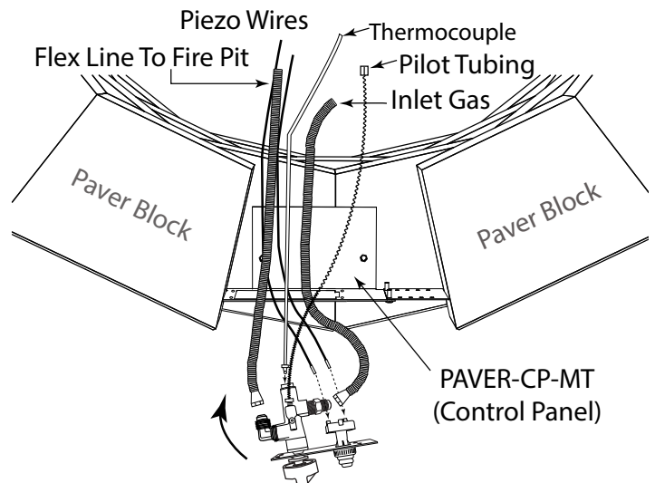
Fig. 7 Installing control panel into PAVER-CP-MT mounting plate.
