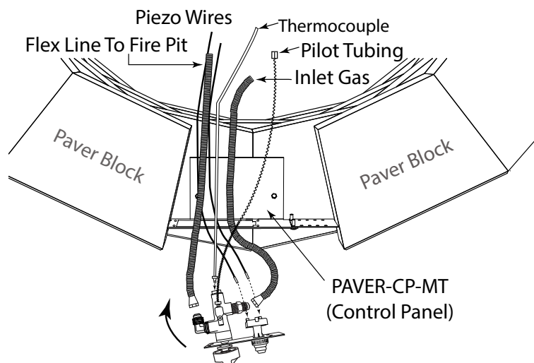
Fig. 6 Installing control panel into PAVER-CP-MT mounting plate.
