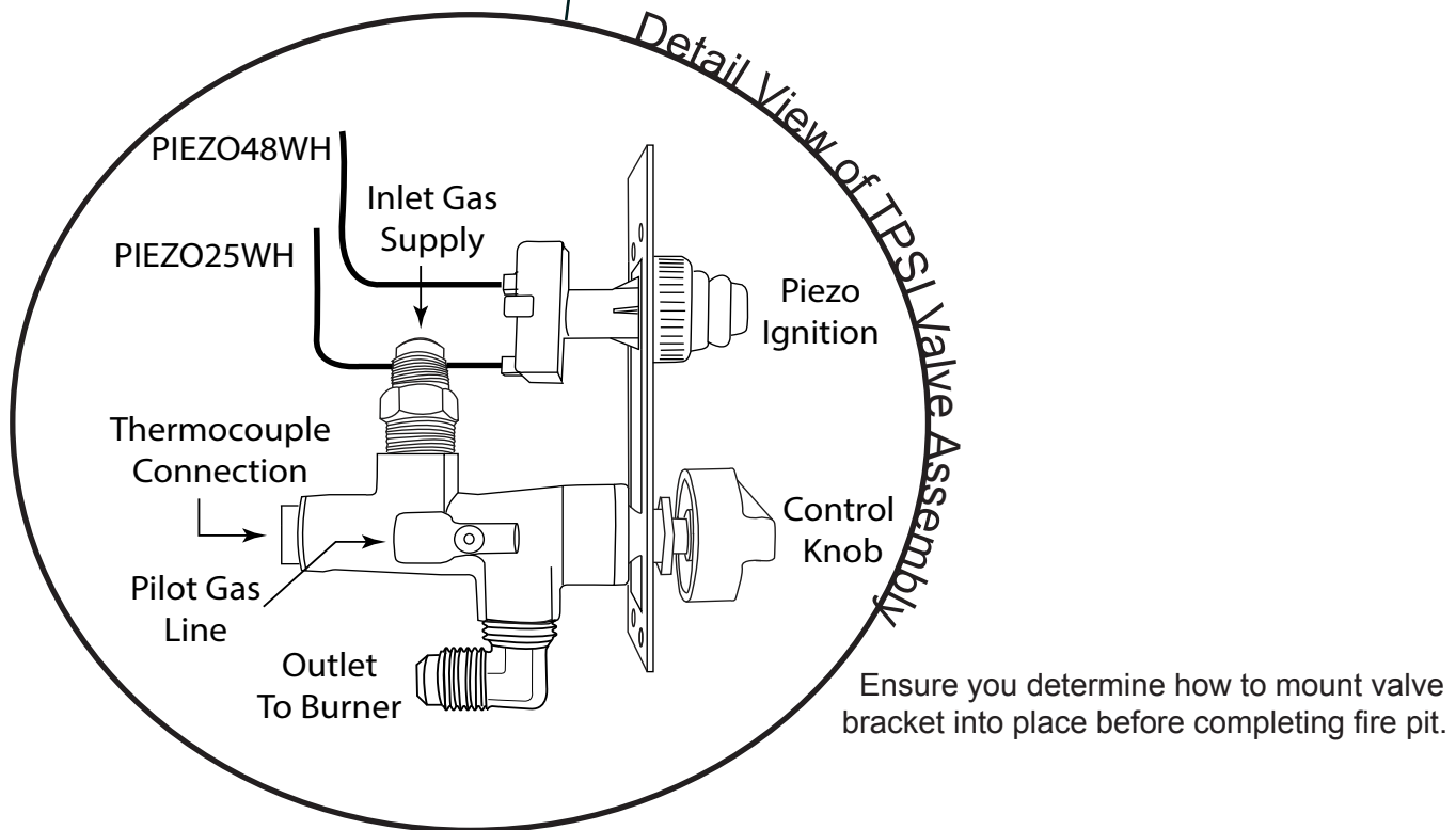
Fig. 11 Typical installation.
