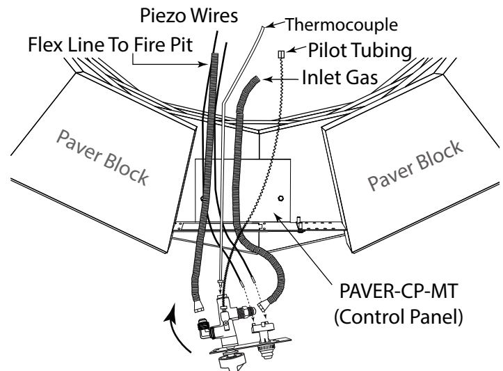
Fig. 5 Installing control panel into PAVER-CP-MT mounting plate.
