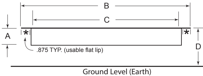
Fig. 1 Burner pan specifications.
