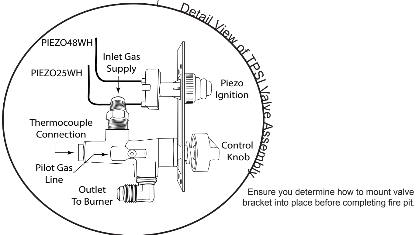
Fig. 13 Typical installation.
