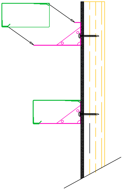
INSTALLED MANTEL SIDE VIEW
