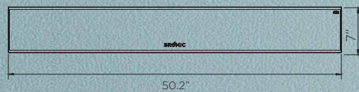
3400W Dimensions:
